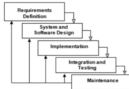
Figure 1. Waterfall method.
